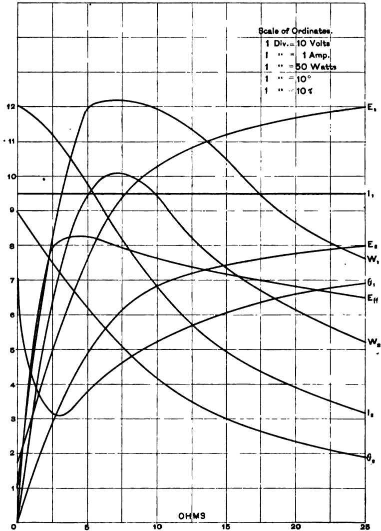
FIG. 14.—Constant Current, Step Down, Arm at 180°.
